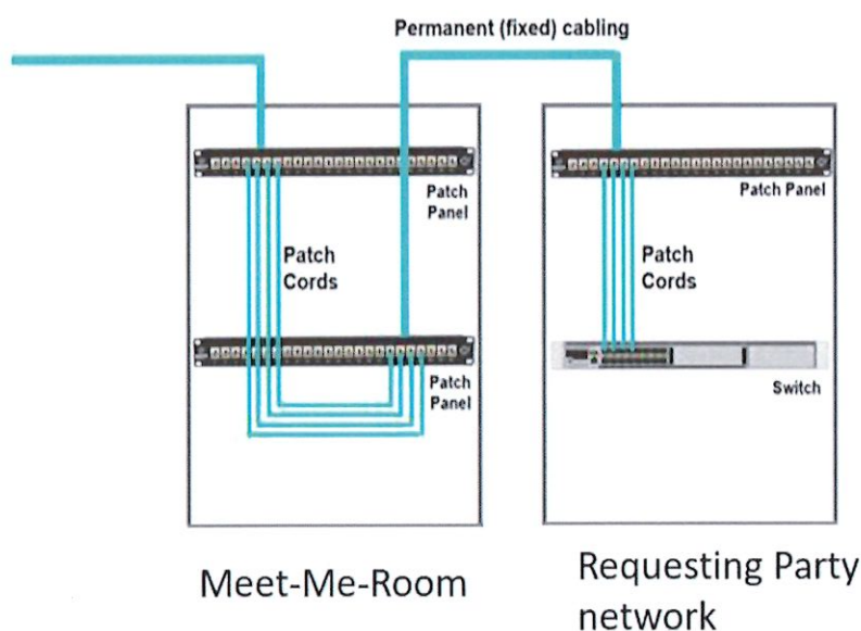
Figure 1: Generic representation of Patching
